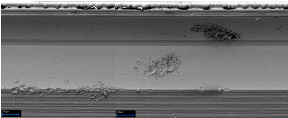
Figure 2: Post-test analysis of a sliping (arcing)
